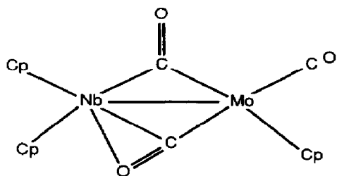
Fig. 3. Structure of 2.37 .
