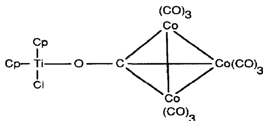
Fig. 1. Structure of 2.8 .
