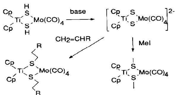
Fig. 28. Reactions of 7.7 .
