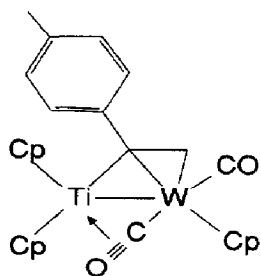
Fig. 17. Structure of 3.13 .
