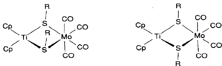
Fig. 26. Cisoid and transoid conformers of \text{Cp}_2\text{Ti}(\mu\text{-SR})_2\text{Mo}(\text{CO})_4 .
