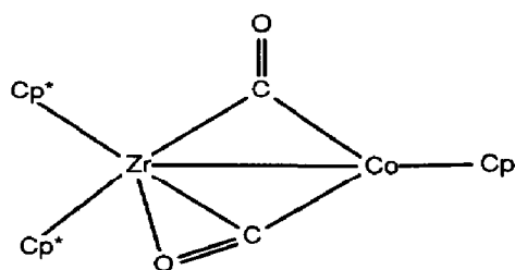
Fig. 10. Structure of 2.30.
