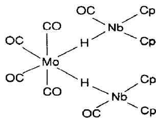
Fig. 20. Structure of 4.9 .
